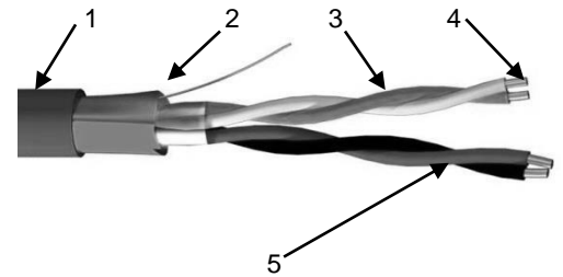
Figure 1. Câble KNX 2 x 2 x 0.8mm
