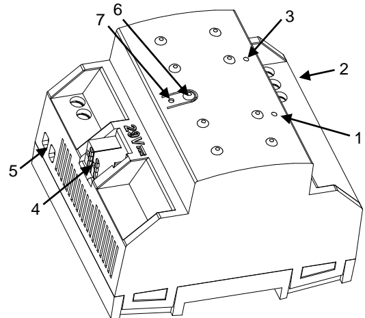
Figure 1: ZPS320MPA110 power supply
