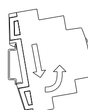
Removing Power Supply from DIN rail:
