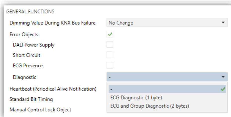
Figure 8. Error Objects
