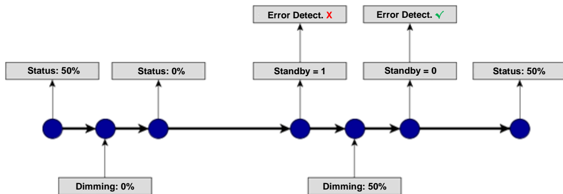
Figure 18. Standby mode action sequence
