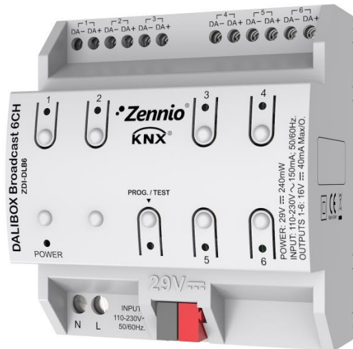
Figura 1. DALIBOX Broadcast 6CH
