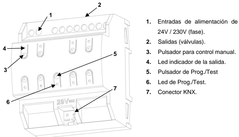
Figura 1. HeatingBOX 230V / 24V 8X.
