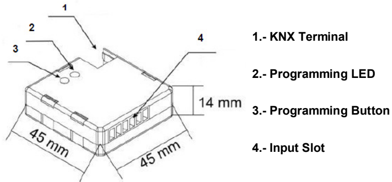
Figure 2 Element scheme.
