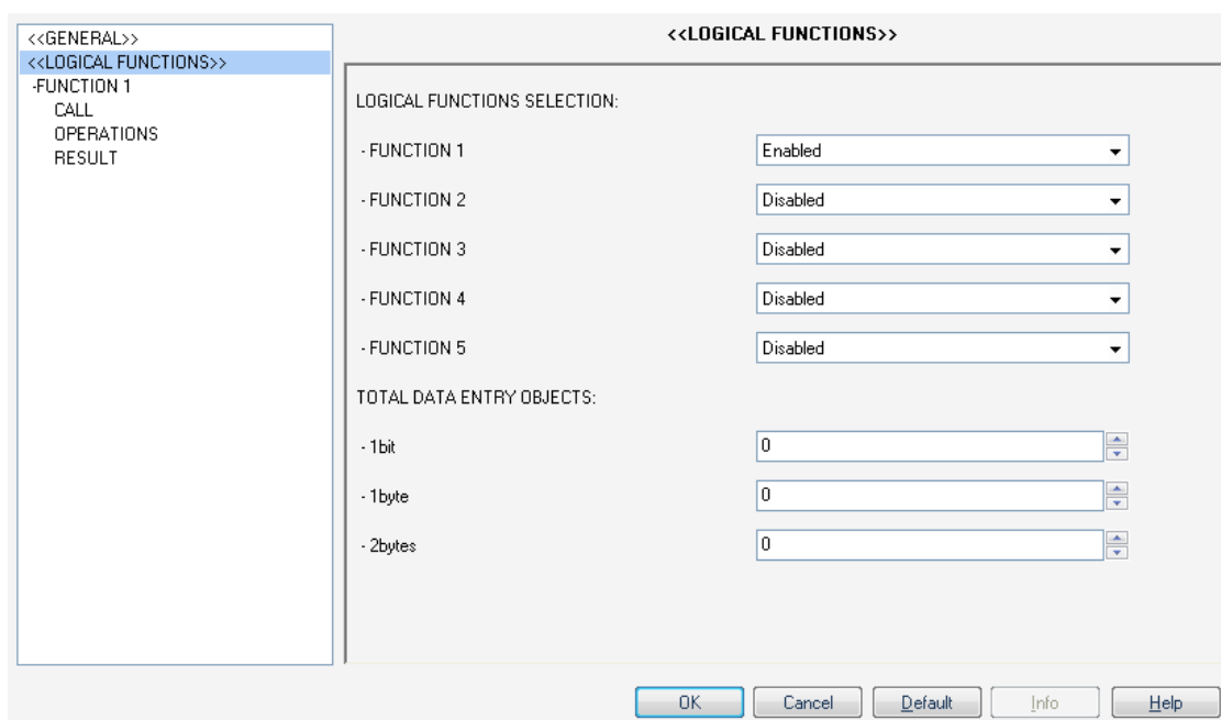
Figure 12 Logical Functions.
