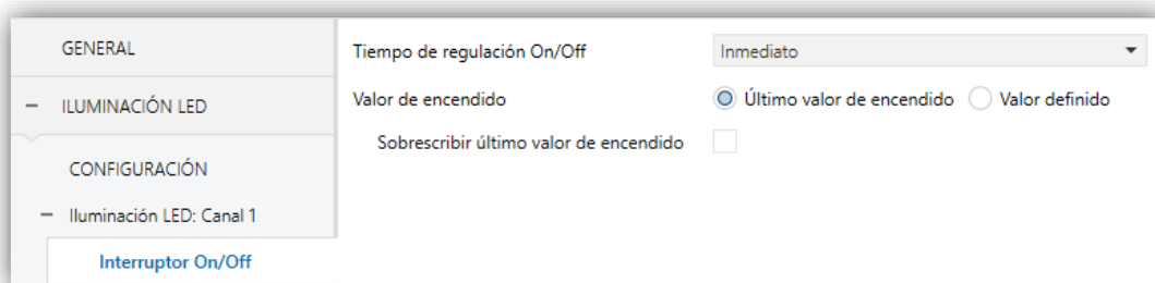
Figura 8. Interruptor On/Off.
