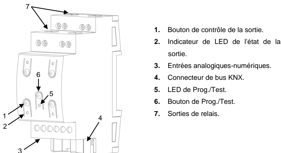
Figure 1. MINIBOX 45 v2. Éléments.
