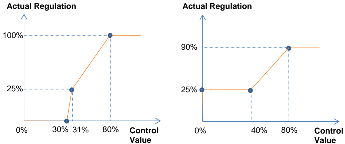
Figure 10. Custom Control Curves.
