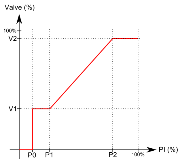
Figure 21. Control order scaling diagram
