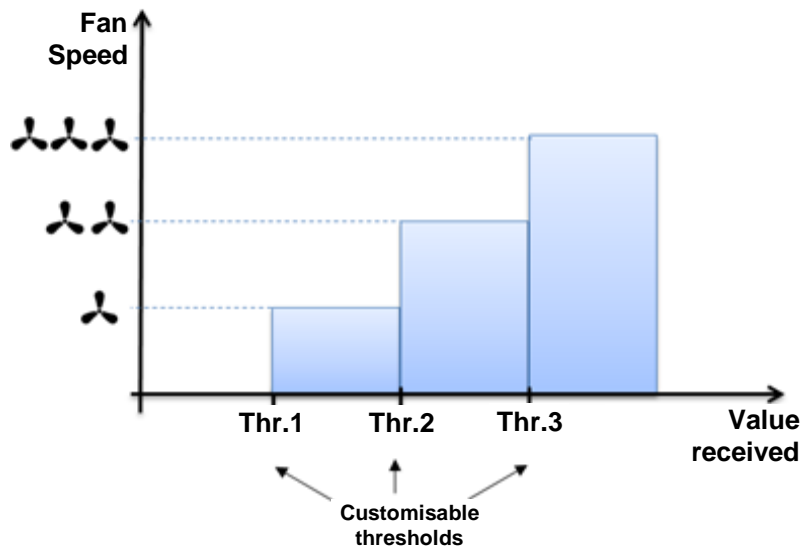
Figure 17. Thresholds, value received and fan speed
