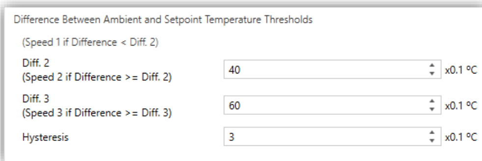
Figure 14. Automatic Fan Control. Temperature Difference
