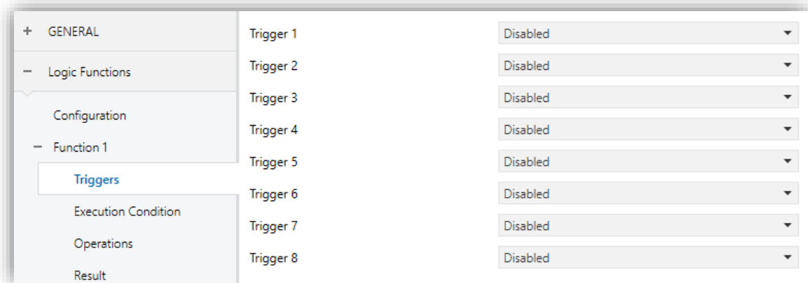
Figure 4. "Triggers" Tab
