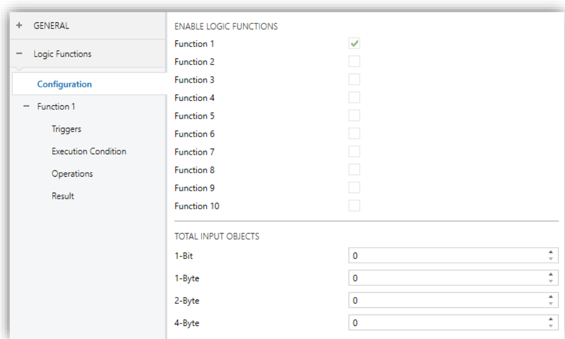
Figure 3. Function 1 enabled.
