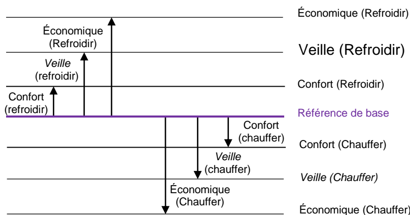
Figure 8. Diagramme de consignes relatives.
